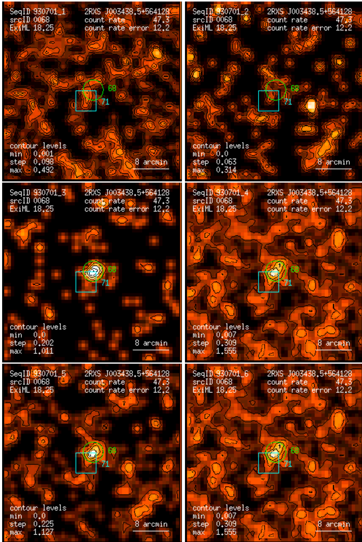
Figure 68: RASS 930701: detection 0068: band rate images, Gaussian filter: (1) PSPC channels 11 – 41, (2) 52 – 90, (3) 91 – 201, (4) 11 – 235, (5) 52 – 201, (6) 11 – 201. Broad band rates in counts/ks. Band rate contour levels in counts/ks/arcmin 2 .
