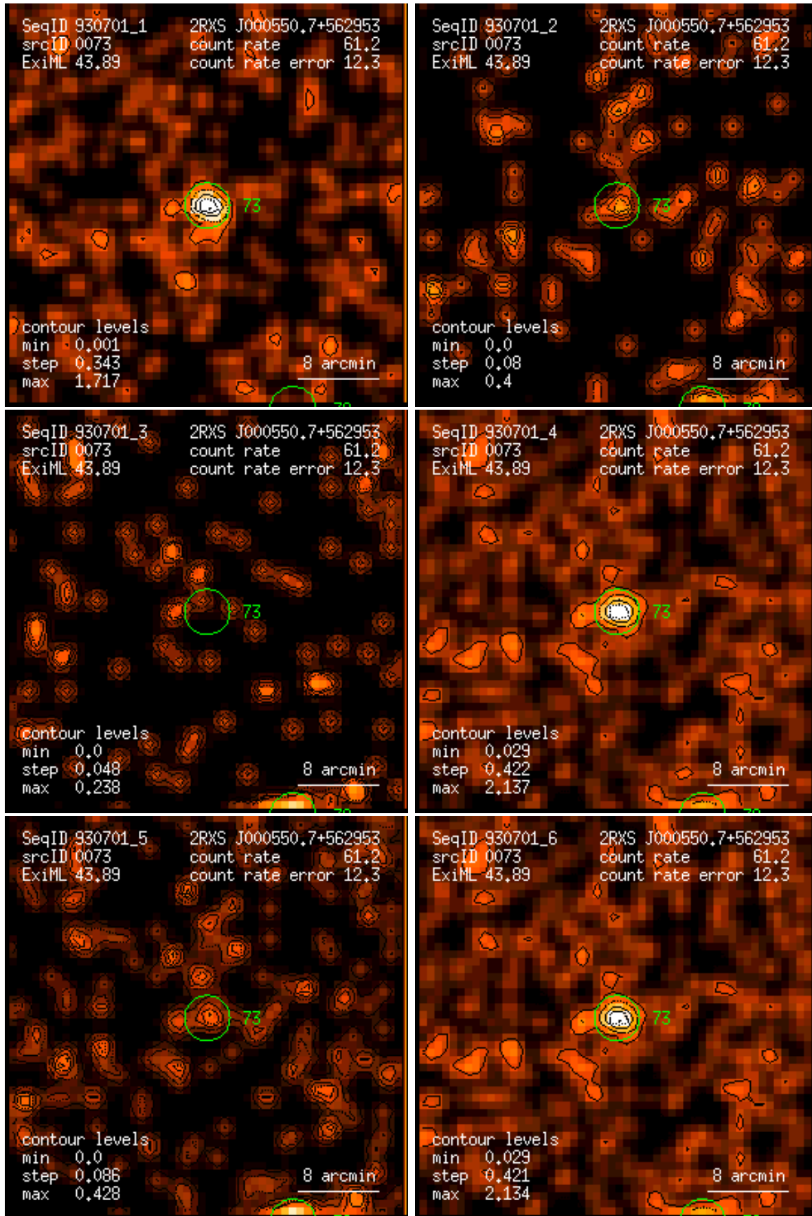
Figure 73: RASS 930701: detection 0073: band rate images, Gaussian filter: (1) PSPC channels 11 – 41, (2) 52 – 90, (3) 91 – 201, (4) 11 – 235, (5) 52 – 201, (6) 11 – 201. Broad band rates in counts/ks. Band rate contour levels in counts/ks/arcmin 2 .
