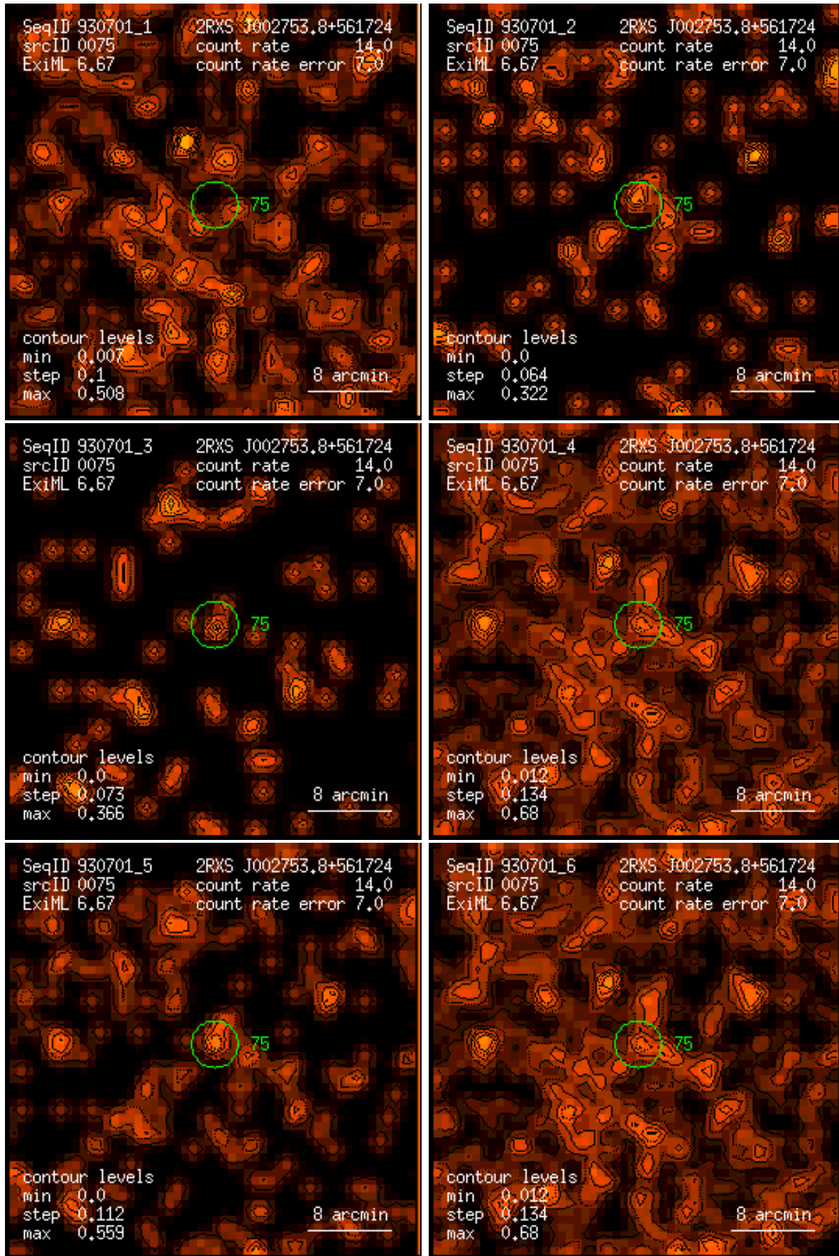
Figure 75: RASS 930701: detection 0075: band rate images, Gaussian filter: (1) PSPC channels 11 – 41, (2) 52 – 90, (3) 91 – 201, (4) 11 – 235, (5) 52 – 201, (6) 11 – 201. Broad band rates in counts/ks. Band rate contour levels in counts/ks/arcmin 2 .
