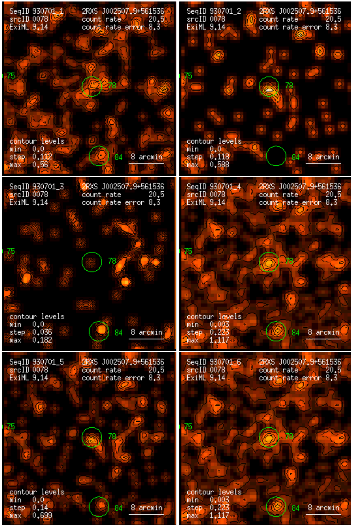
Figure 78: RASS 930701: detection 0078: band rate images, Gaussian filter: (1) PSPC channels 11 – 41, (2) 52 – 90, (3) 91 – 201, (4) 11 – 235, (5) 52 – 201, (6) 11 – 201. Broad band rates in counts/ks. Band rate contour levels in counts/ks/arcmin 2 .
