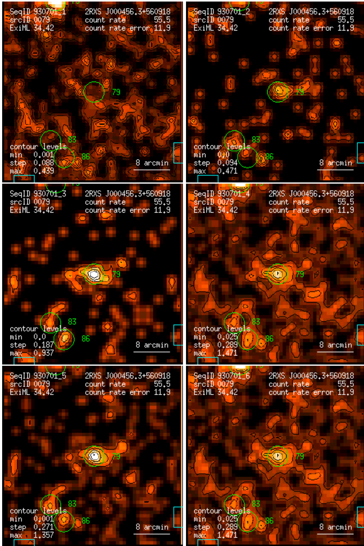
Figure 79: RASS 930701: detection 0079: band rate images, Gaussian filter: (1) PSPC channels 11 – 41, (2) 52 – 90, (3) 91 – 201, (4) 11 – 235, (5) 52 – 201, (6) 11 – 201. Broad band rates in counts/ks. Band rate contour levels in counts/ks/arcmin 2 .
