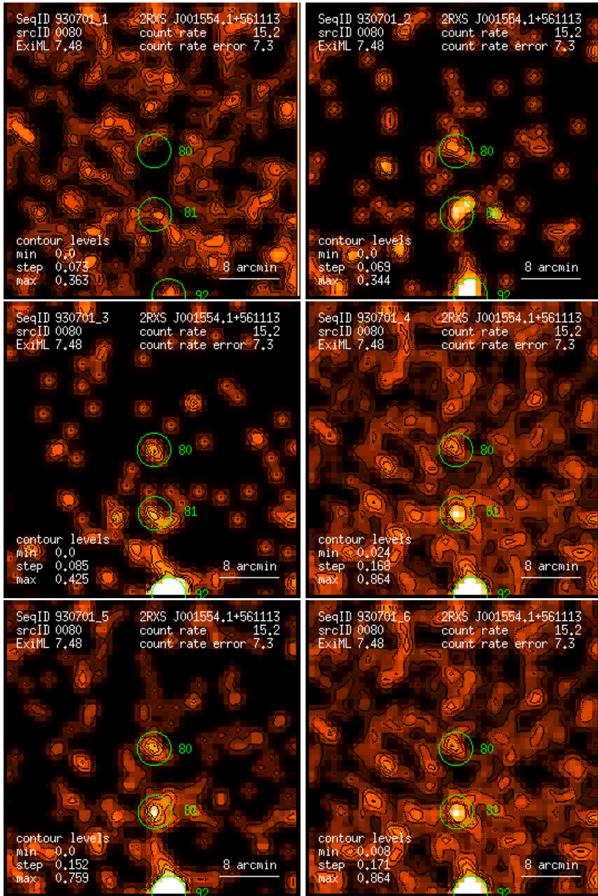
Figure 80: RASS 930701: detection 0080: band rate images, Gaussian filter: (1) PSPC channels 11 – 41, (2) 52 – 90, (3) 91 – 201, (4) 11 – 235, (5) 52 – 201, (6) 11 – 201. Broad band rates in counts/ks. Band rate contour levels in counts/ks/arcmin 2 .
