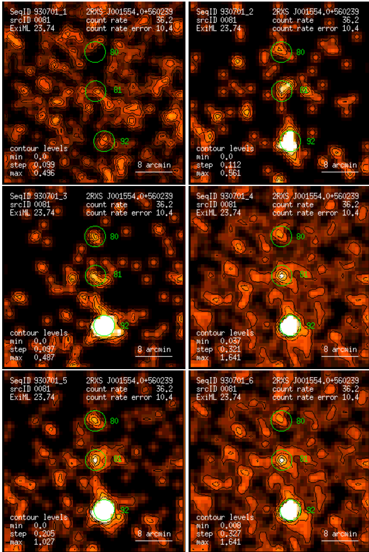
Figure 81: RASS 930701: detection 0081: band rate images, Gaussian filter: (1) PSPC channels 11 – 41, (2) 52 – 90, (3) 91 – 201, (4) 11 – 235, (5) 52 – 201, (6) 11 – 201. Broad band rates in counts/ks. Band rate contour levels in counts/ks/arcmin 2 .
