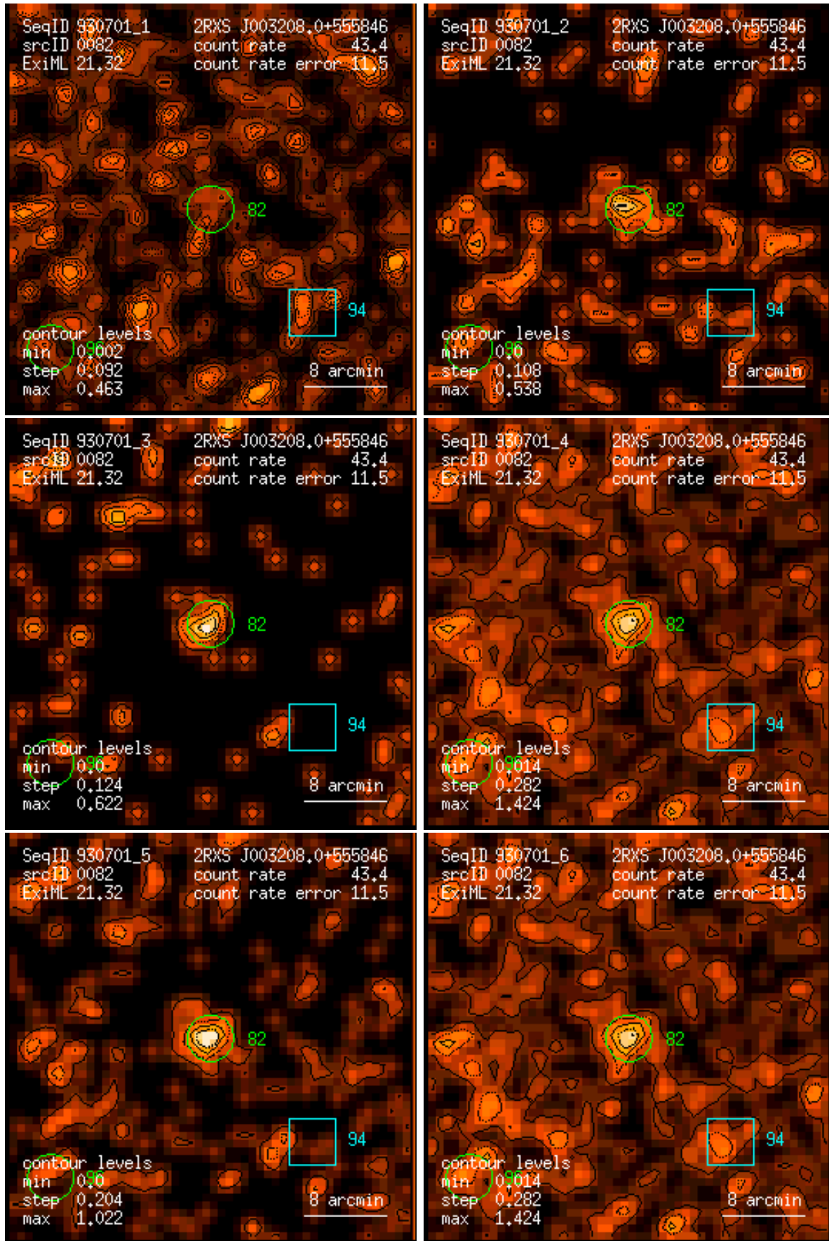
Figure 82: RASS 930701: detection 0082: band rate images, Gaussian filter: (1) PSPC channels 11 – 41, (2) 52 – 90, (3) 91 – 201, (4) 11 – 235, (5) 52 – 201, (6) 11 – 201. Broad band rates in counts/ks. Band rate contour levels in counts/ks/arcmin 2 .
