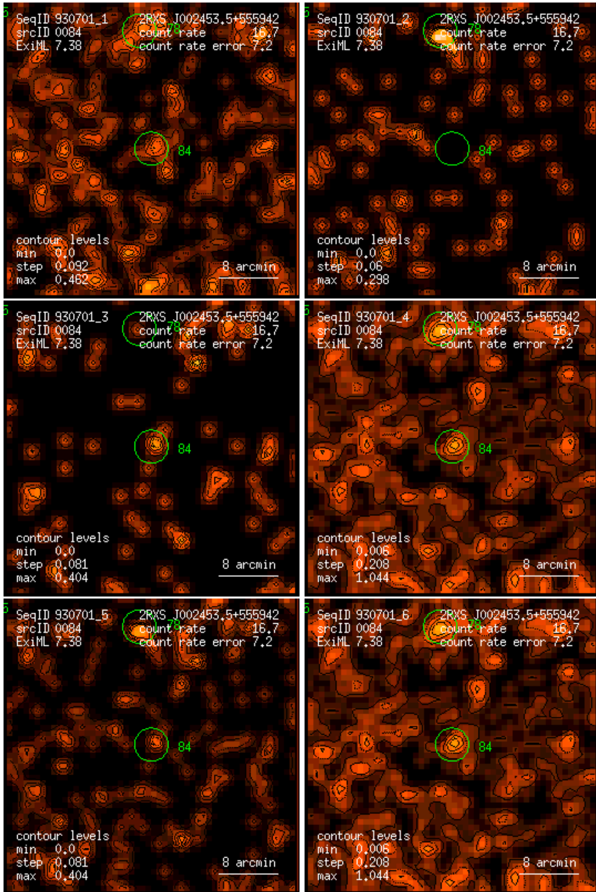
Figure 84: RASS 930701: detection 0084: band rate images, Gaussian filter: (1) PSPC channels 11 – 41, (2) 52 – 90, (3) 91 – 201, (4) 11 – 235, (5) 52 – 201, (6) 11 – 201. Broad band rates in counts/ks. Band rate contour levels in counts/ks/arcmin 2 .
