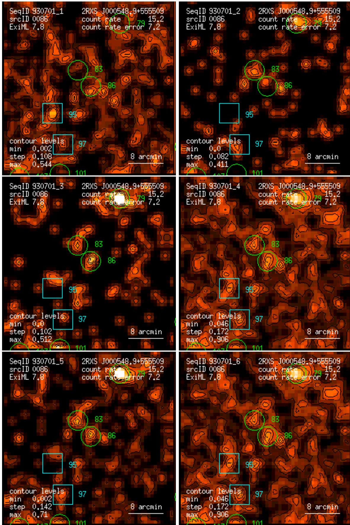
Figure 86: RASS 930701: detection 0086: band rate images, Gaussian filter: (1) PSPC channels 11 – 41, (2) 52 – 90, (3) 91 – 201, (4) 11 – 235, (5) 52 – 201, (6) 11 – 201. Broad band rates in counts/ks. Band rate contour levels in counts/ks/arcmin 2 .
