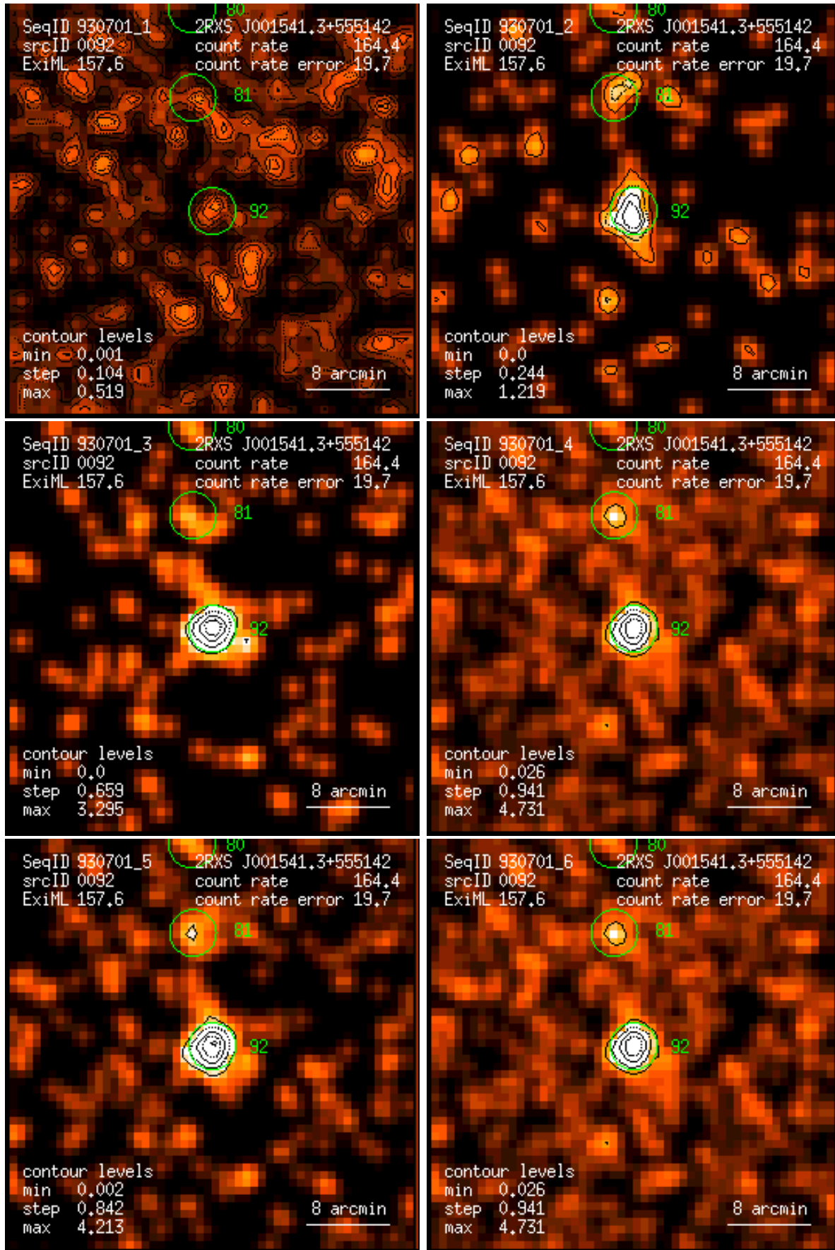
Figure 92: RASS 930701: detection 0092: band rate images, Gaussian filter: (1) PSPC channels 11 – 41, (2) 52 – 90, (3) 91 – 201, (4) 11 – 235, (5) 52 – 201, (6) 11 – 201. Broad band rates in counts/ks. Band rate contour levels in counts/ks/arcmin 2 .
