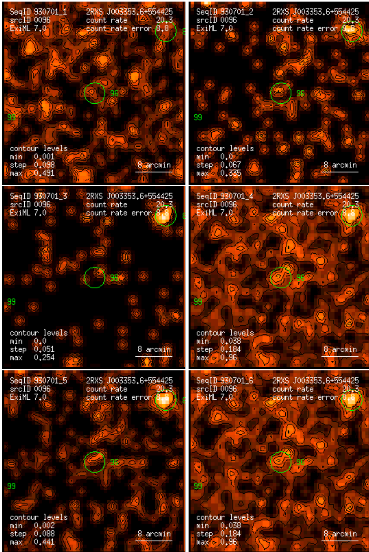
Figure 96: RASS 930701: detection 0096: band rate images, Gaussian filter: (1) PSPC channels 11 – 41, (2) 52 – 90, (3) 91 – 201, (4) 11 – 235, (5) 52 – 201, (6) 11 – 201. Broad band rates in counts/ks. Band rate contour levels in counts/ks/arcmin 2 .
