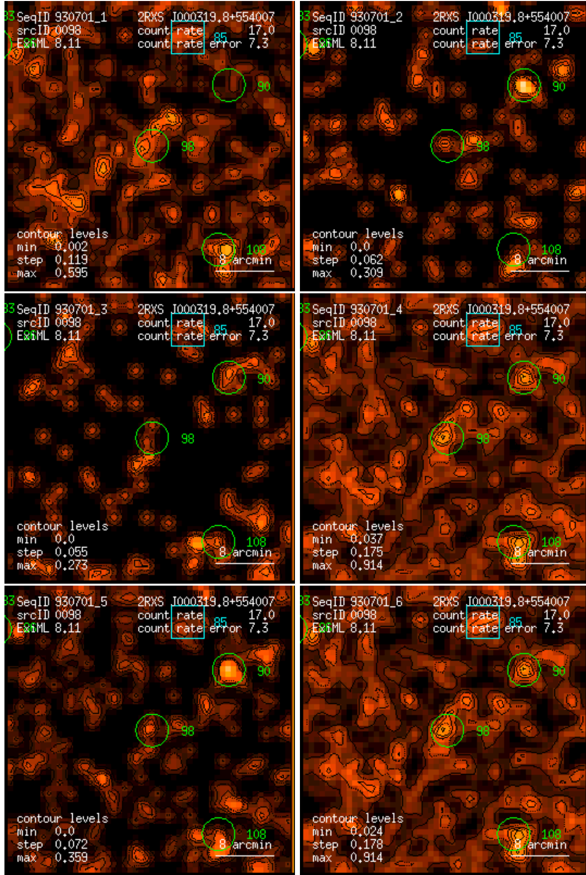
Figure 98: RASS 930701: detection 0098: band rate images, Gaussian filter: (1) PSPC channels 11 – 41, (2) 52 – 90, (3) 91 – 201, (4) 11 – 235, (5) 52 – 201, (6) 11 – 201. Broad band rates in counts/ks. Band rate contour levels in counts/ks/arcmin 2 .
