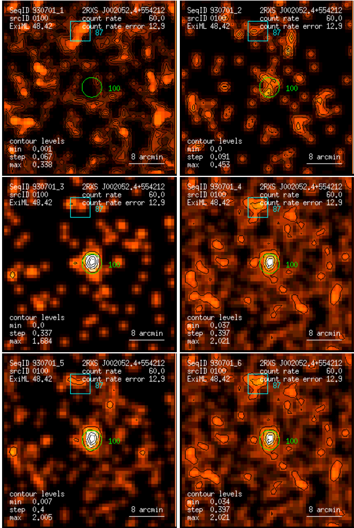
Figure 100: RASS 930701: detection 0100: band rate images, Gaussian filter: (1) PSPC channels 11 – 41, (2) 52 – 90, (3) 91 – 201, (4) 11 – 235, (5) 52 – 201, (6) 11 – 201. Broad band rates in counts/ks. Band rate contour levels in counts/ks/arcmin 2 .
