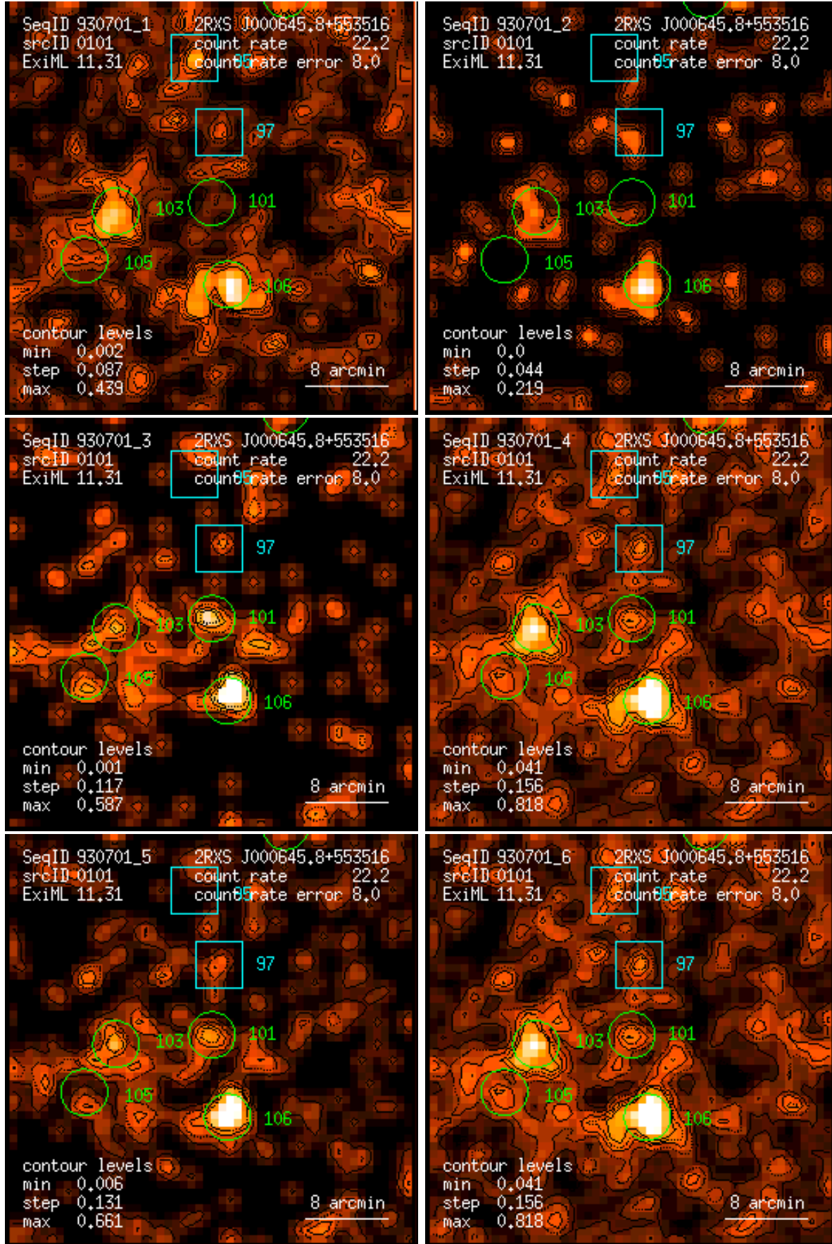
Figure 101: RASS 930701: detection 0101: band rate images, Gaussian filter: (1) PSPC channels 11 – 41, (2) 52 – 90, (3) 91 – 201, (4) 11 – 235, (5) 52 – 201, (6) 11 – 201. Broad band rates in counts/ks. Band rate contour levels in counts/ks/arcmin 2 .
