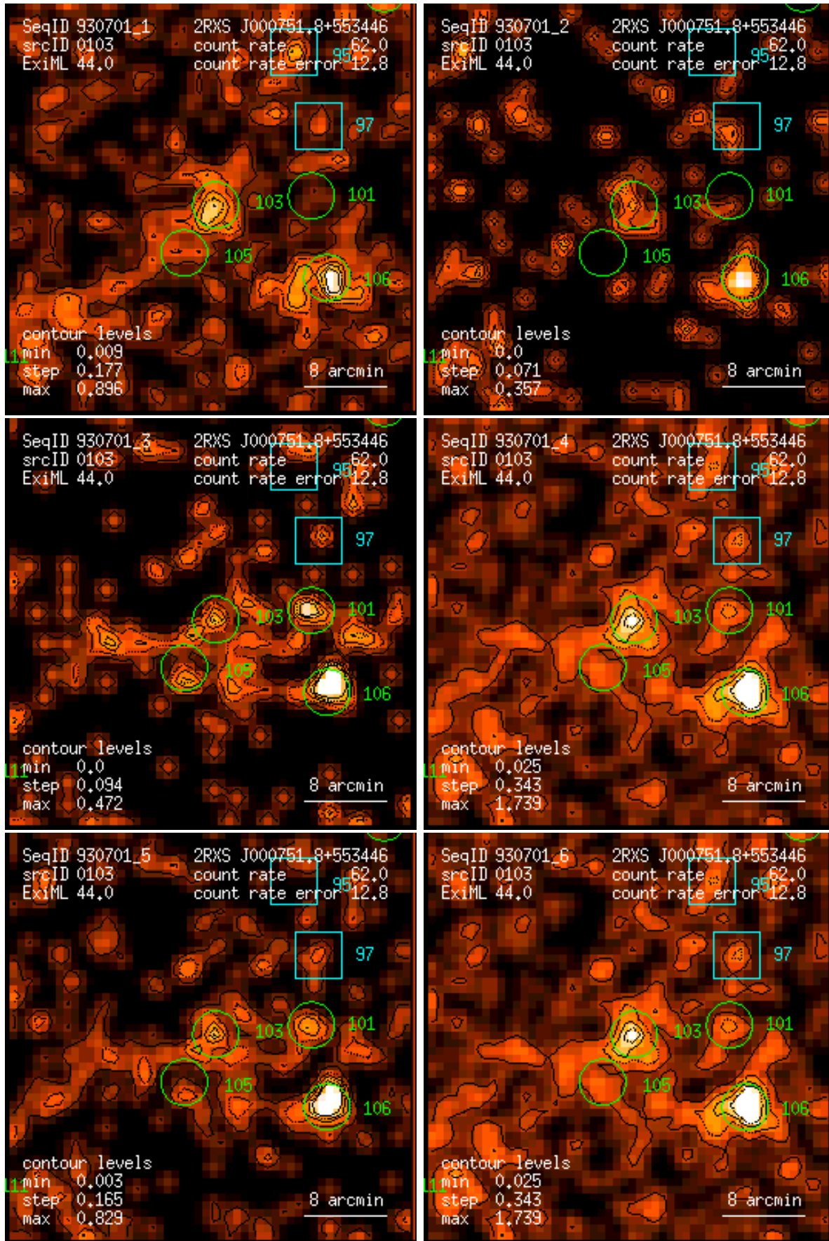
Figure 103: RASS 930701: detection 0103: band rate images, Gaussian filter: (1) PSPC channels 11 – 41, (2) 52 – 90, (3) 91 – 201, (4) 11 – 235, (5) 52 – 201, (6) 11 – 201. Broad band rates in counts/ks. Band rate contour levels in counts/ks/arcmin 2 .
