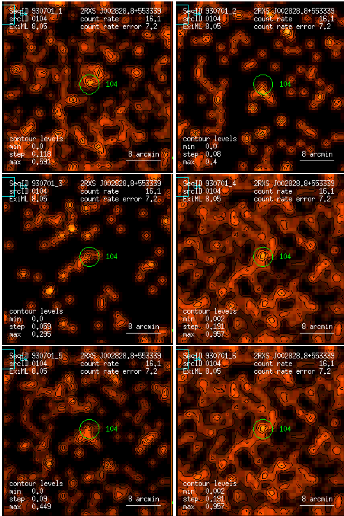
Figure 104: RASS 930701: detection 0104: band rate images, Gaussian filter: (1) PSPC channels 11 – 41, (2) 52 – 90, (3) 91 – 201, (4) 11 – 235, (5) 52 – 201, (6) 11 – 201. Broad band rates in counts/ks. Band rate contour levels in counts/ks/arcmin 2 .
