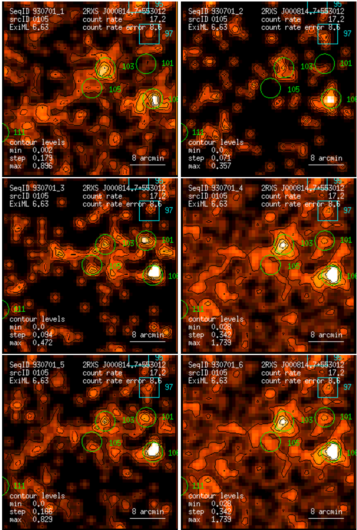
Figure 105: RASS 930701: detection 0105: band rate images, Gaussian filter: (1) PSPC channels 11 – 41, (2) 52 – 90, (3) 91 – 201, (4) 11 – 235, (5) 52 – 201, (6) 11 – 201. Broad band rates in counts/ks. Band rate contour levels in counts/ks/arcmin 2 .
