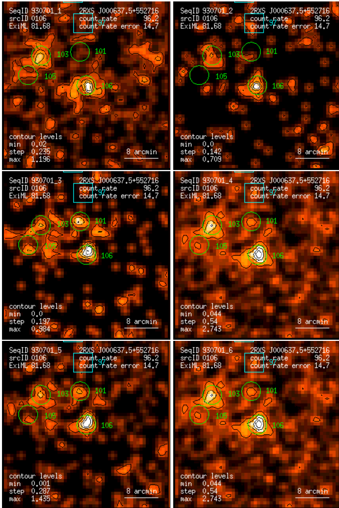
Figure 106: RASS 930701: detection 0106: band rate images, Gaussian filter: (1) PSPC channels 11 – 41, (2) 52 – 90, (3) 91 – 201, (4) 11 – 235, (5) 52 – 201, (6) 11 – 201. Broad band rates in counts/ks. Band rate contour levels in counts/ks/arcmin 2 .
