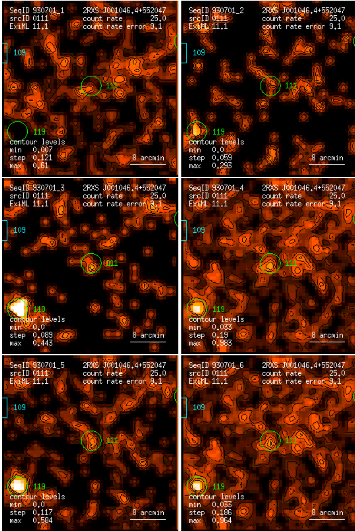
Figure 111: RASS 930701: detection 0111: band rate images, Gaussian filter: (1) PSPC channels 11 – 41, (2) 52 – 90, (3) 91 – 201, (4) 11 – 235, (5) 52 – 201, (6) 11 – 201. Broad band rates in counts/ks. Band rate contour levels in counts/ks/arcmin 2 .
