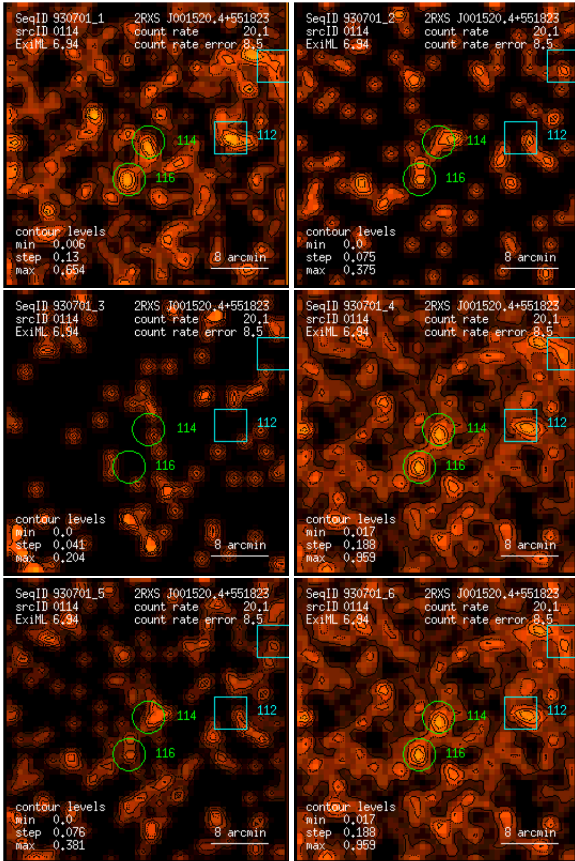
Figure 114: RASS 930701: detection 0114: band rate images, Gaussian filter: (1) PSPC channels 11 – 41, (2) 52 – 90, (3) 91 – 201, (4) 11 – 235, (5) 52 – 201, (6) 11 – 201. Broad band rates in counts/ks. Band rate contour levels in counts/ks/arcmin 2 .
