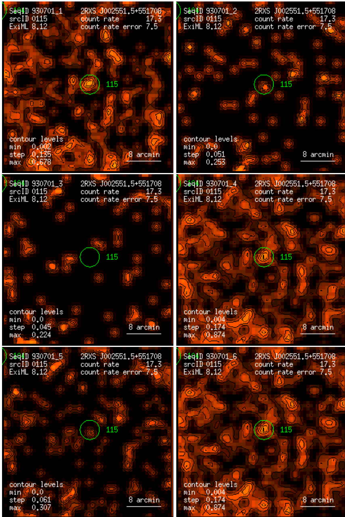
Figure 115: RASS 930701: detection 0115: band rate images, Gaussian filter: (1) PSPC channels 11 – 41, (2) 52 – 90, (3) 91 – 201, (4) 11 – 235, (5) 52 – 201, (6) 11 – 201. Broad band rates in counts/ks. Band rate contour levels in counts/ks/arcmin 2 .
