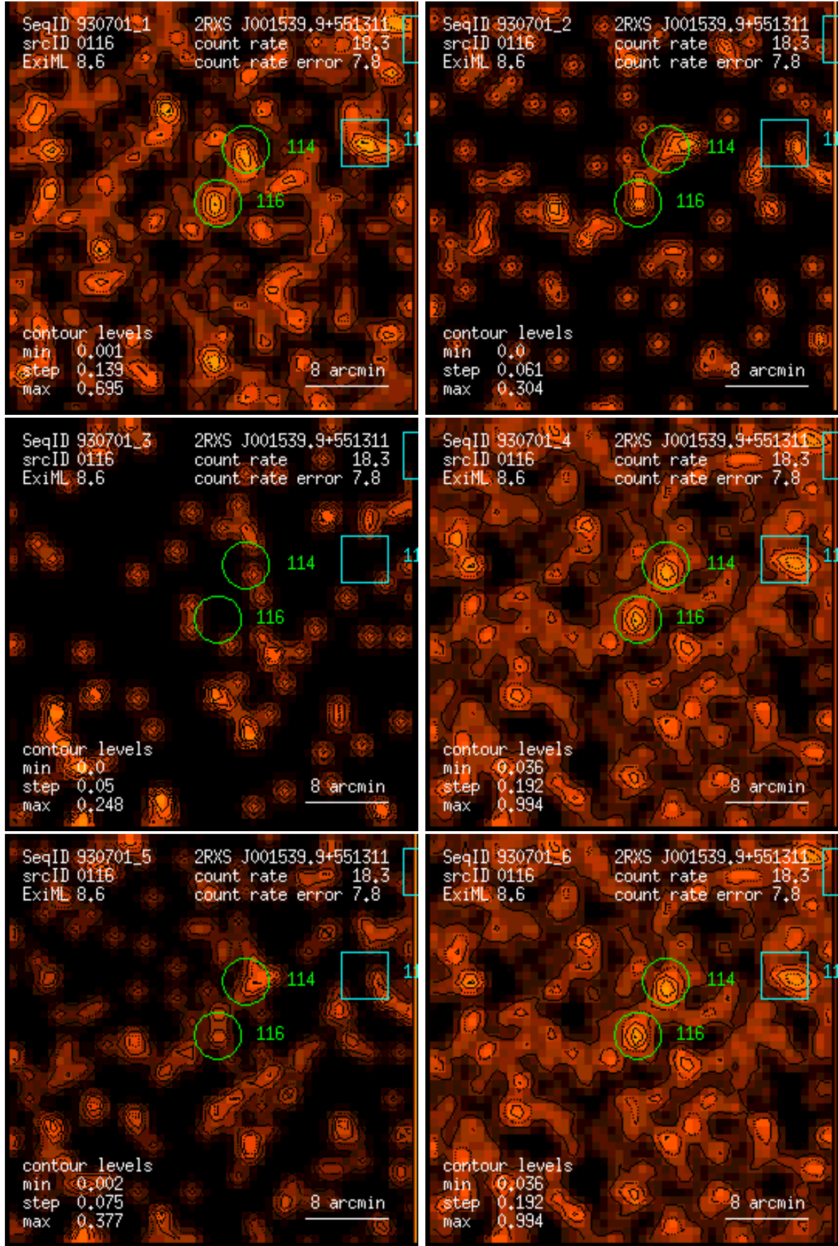
Figure 116: RASS 930701: detection 0116: band rate images, Gaussian filter: (1) PSPC channels 11 – 41, (2) 52 – 90, (3) 91 – 201, (4) 11 – 235, (5) 52 – 201, (6) 11 – 201. Broad band rates in counts/ks. Band rate contour levels in counts/ks/arcmin 2 .
