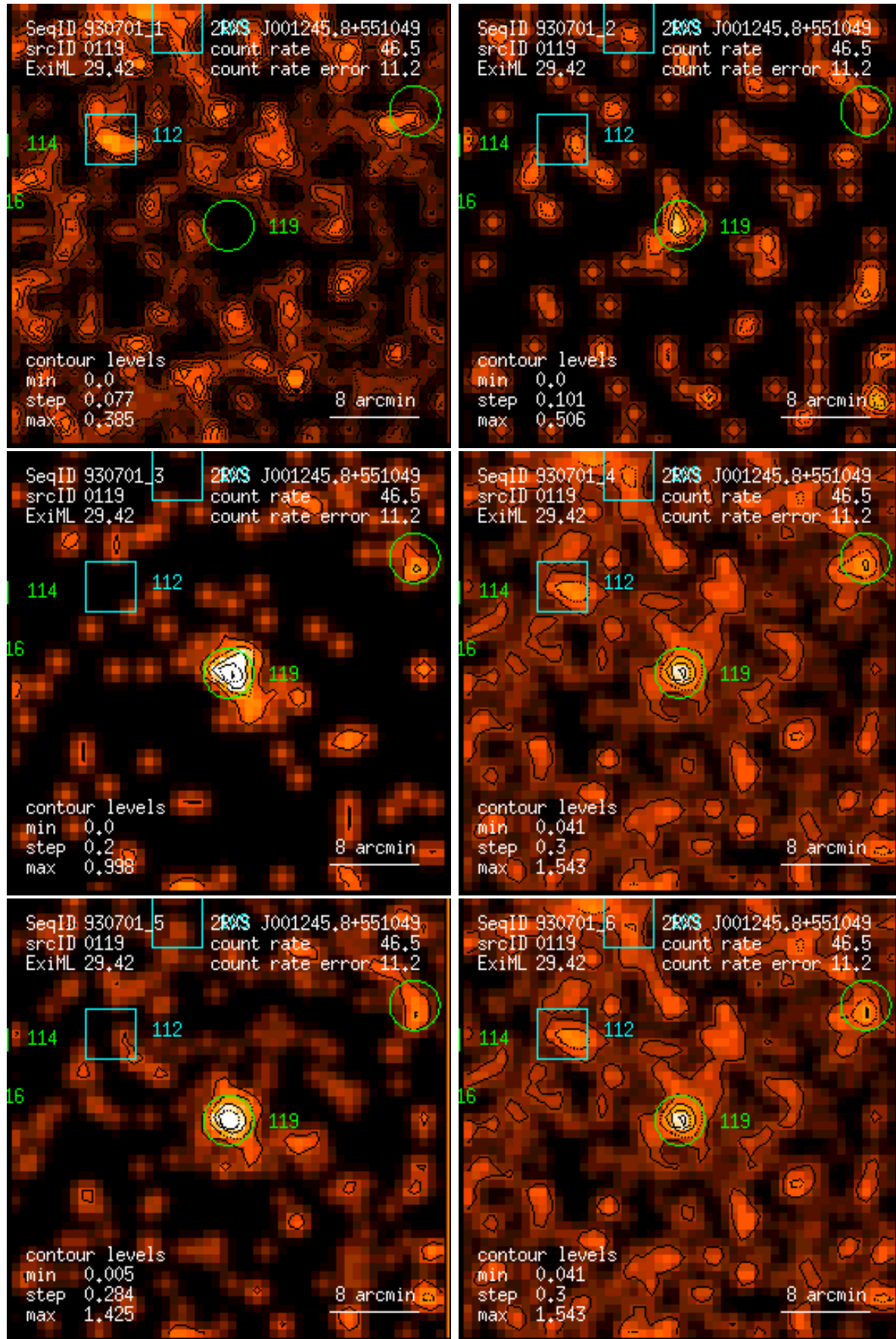
Figure 119: RASS 930701: detection 0119: band rate images, Gaussian filter: (1) PSPC channels 11 – 41, (2) 52 – 90, (3) 91 – 201, (4) 11 – 235, (5) 52 – 201, (6) 11 – 201. Broad band rates in counts/ks. Band rate contour levels in counts/ks/arcmin 2 .
