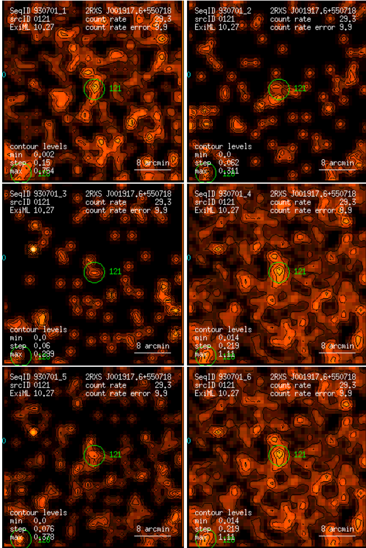
Figure 121: RASS 930701: detection 0121: band rate images, Gaussian filter: (1) PSPC channels 11 – 41, (2) 52 – 90, (3) 91 – 201, (4) 11 – 235, (5) 52 – 201, (6) 11 – 201. Broad band rates in counts/ks. Band rate contour levels in counts/ks/arcmin 2 .
