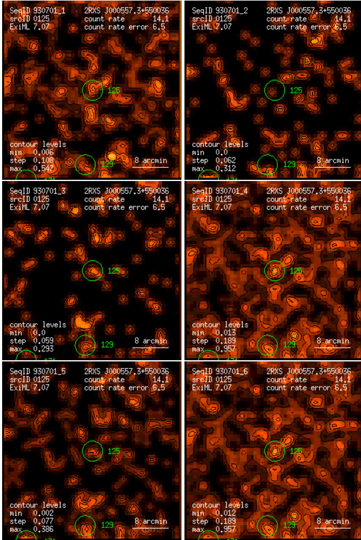
Figure 125: RASS 930701: detection 0125: band rate images, Gaussian filter: (1) PSPC channels 11 – 41, (2) 52 – 90, (3) 91 – 201, (4) 11 – 235, (5) 52 – 201, (6) 11 – 201. Broad band rates in counts/ks. Band rate contour levels in counts/ks/arcmin 2 .
