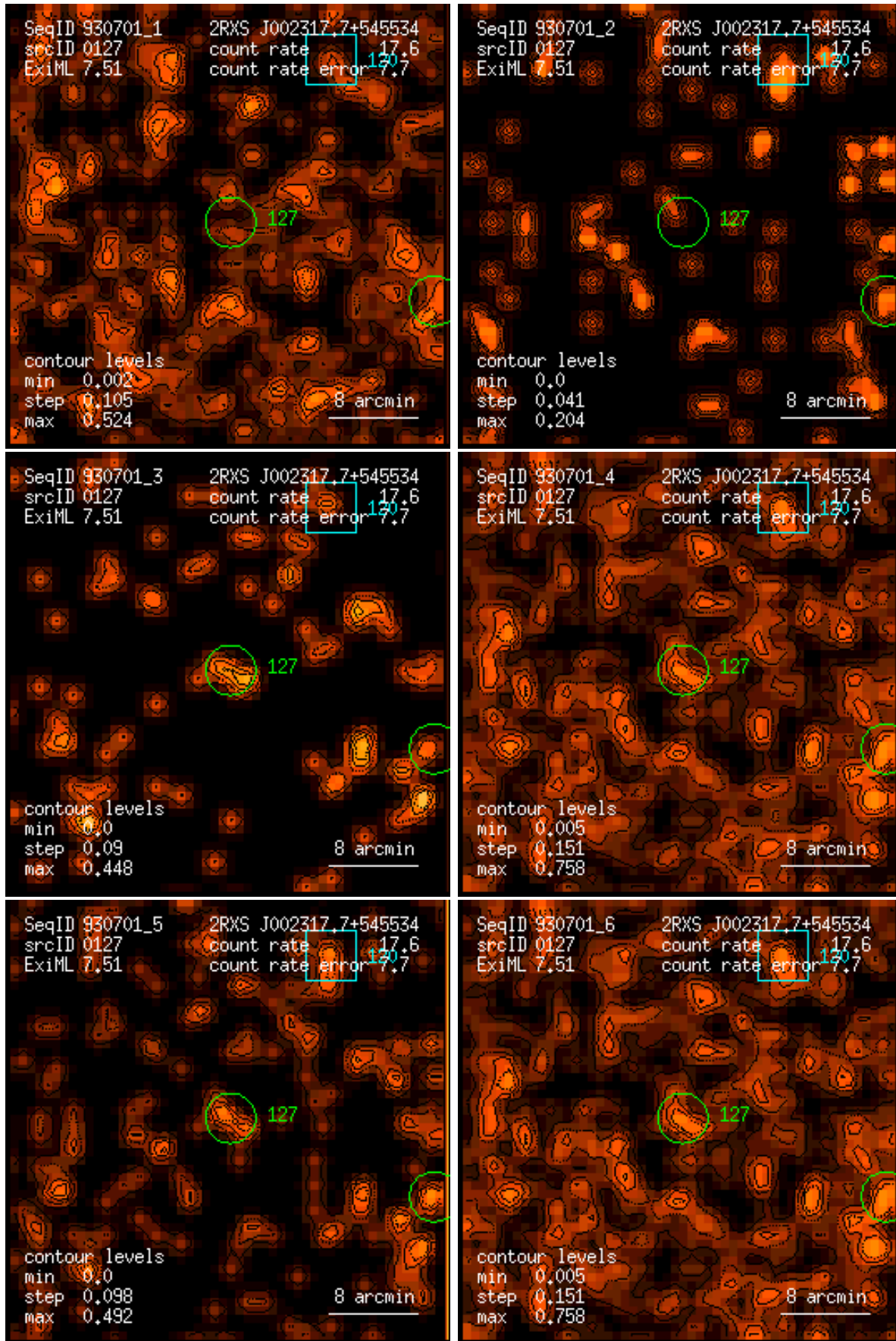
Figure 127: RASS 930701: detection 0127: band rate images, Gaussian filter: (1) PSPC channels 11 – 41, (2) 52 – 90, (3) 91 – 201, (4) 11 – 235, (5) 52 – 201, (6) 11 – 201. Broad band rates in counts/ks. Band rate contour levels in counts/ks/arcmin 2 .
