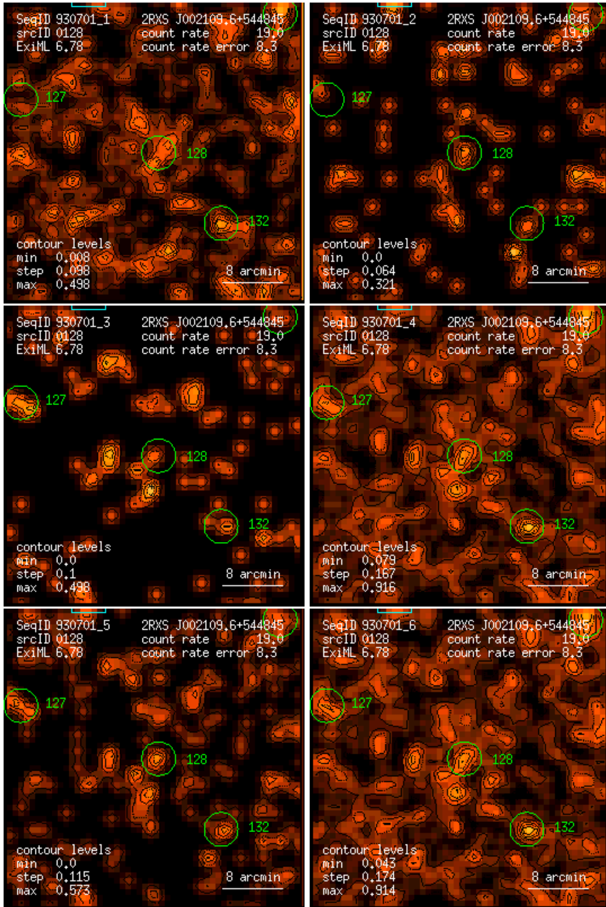
Figure 128: RASS 930701: detection 0128: band rate images, Gaussian filter: (1) PSPC channels 11 – 41, (2) 52 – 90, (3) 91 – 201, (4) 11 – 235, (5) 52 – 201, (6) 11 – 201. Broad band rates in counts/ks. Band rate contour levels in counts/ks/arcmin 2 .
