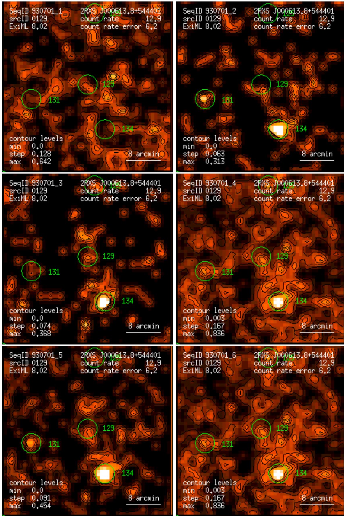
Figure 129: RASS 930701: detection 0129: band rate images, Gaussian filter: (1) PSPC channels 11 – 41, (2) 52 – 90, (3) 91 – 201, (4) 11 – 235, (5) 52 – 201, (6) 11 – 201. Broad band rates in counts/ks. Band rate contour levels in counts/ks/arcmin 2 .
