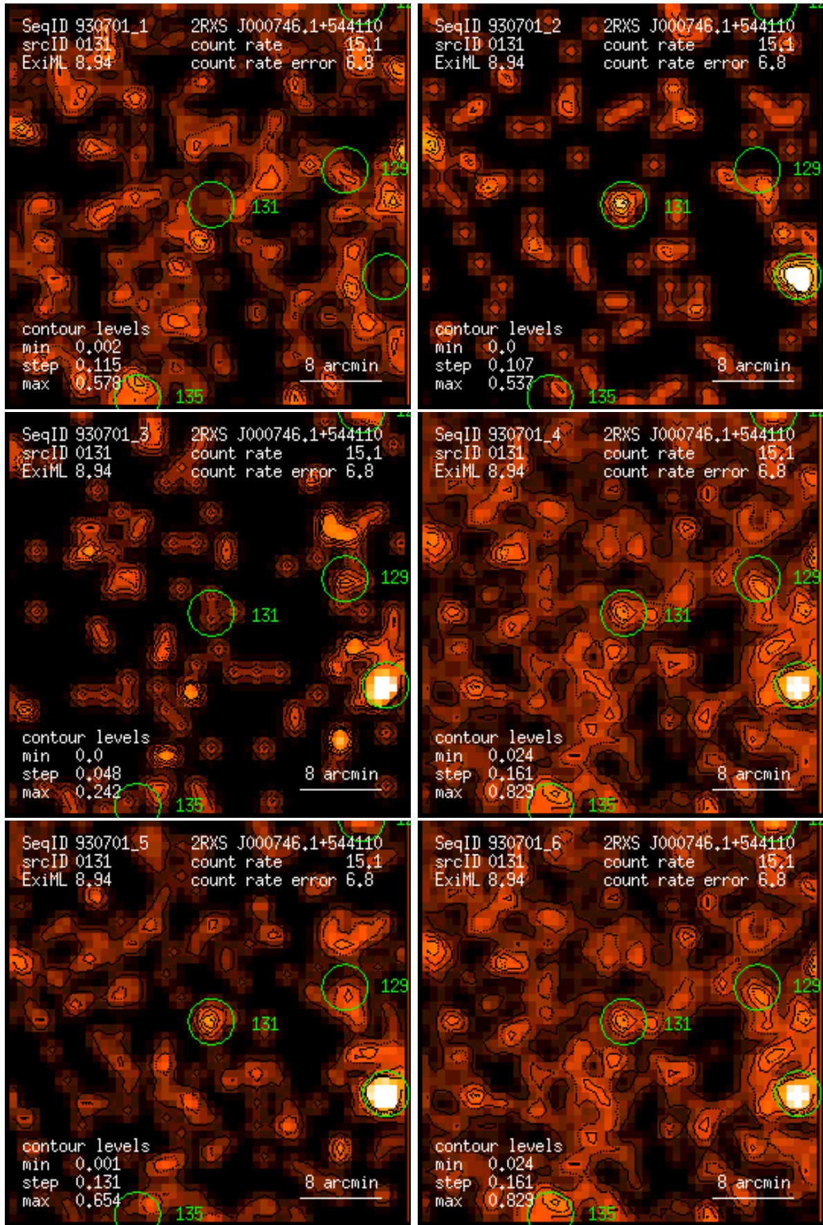
Figure 131: RASS 930701: detection 0131: band rate images, Gaussian filter: (1) PSPC channels 11 – 41, (2) 52 – 90, (3) 91 – 201, (4) 11 – 235, (5) 52 – 201, (6) 11 – 201. Broad band rates in counts/ks. Band rate contour levels in counts/ks/arcmin 2 .
