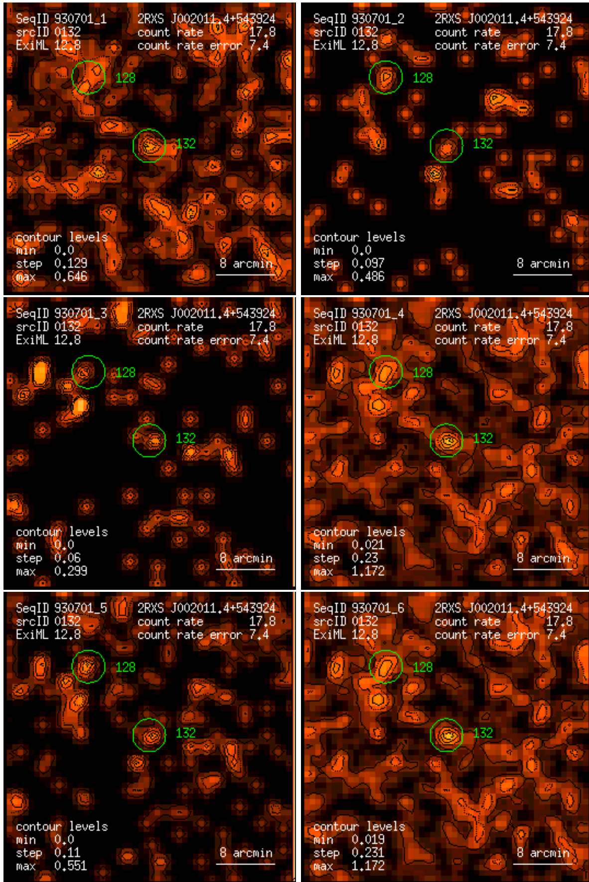
Figure 132: RASS 930701: detection 0132: band rate images, Gaussian filter: (1) PSPC channels 11 – 41, (2) 52 – 90, (3) 91 – 201, (4) 11 – 235, (5) 52 – 201, (6) 11 – 201. Broad band rates in counts/ks. Band rate contour levels in counts/ks/arcmin 2 .
