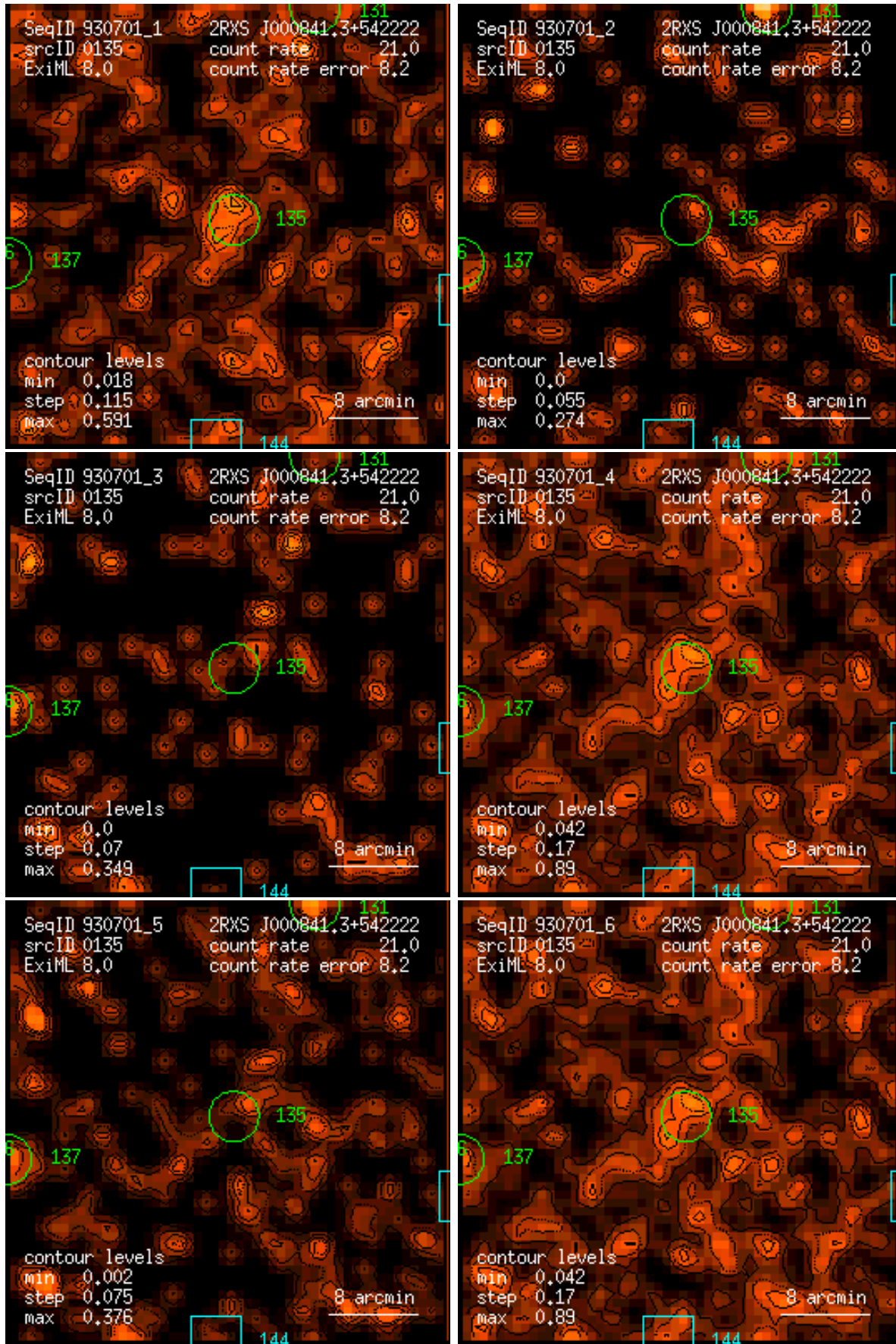
Figure 135: RASS 930701: detection 0135: band rate images, Gaussian filter: (1) PSPC channels 11 – 41, (2) 52 – 90, (3) 91 – 201, (4) 11 – 235, (5) 52 – 201, (6) 11 – 201. Broad band rates in counts/ks. Band rate contour levels in counts/ks/arcmin 2 .
