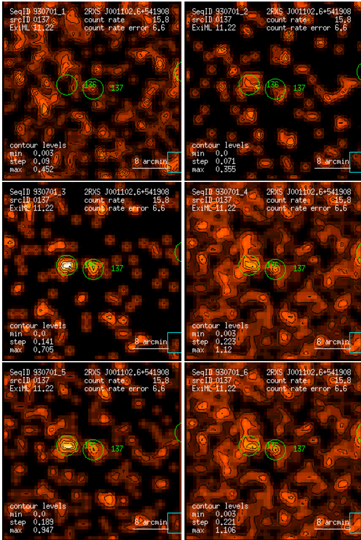
Figure 137: RASS 930701: detection 0137: band rate images, Gaussian filter: (1) PSPC channels 11 – 41, (2) 52 – 90, (3) 91 – 201, (4) 11 – 235, (5) 52 – 201, (6) 11 – 201. Broad band rates in counts/ks. Band rate contour levels in counts/ks/arcmin 2 .
