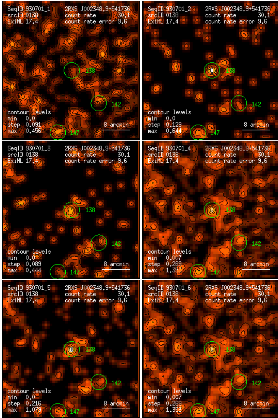
Figure 138: RASS 930701: detection 0138: band rate images, Gaussian filter: (1) PSPC channels 11 – 41, (2) 52 – 90, (3) 91 – 201, (4) 11 – 235, (5) 52 – 201, (6) 11 – 201. Broad band rates in counts/ks. Band rate contour levels in counts/ks/arcmin 2 .
