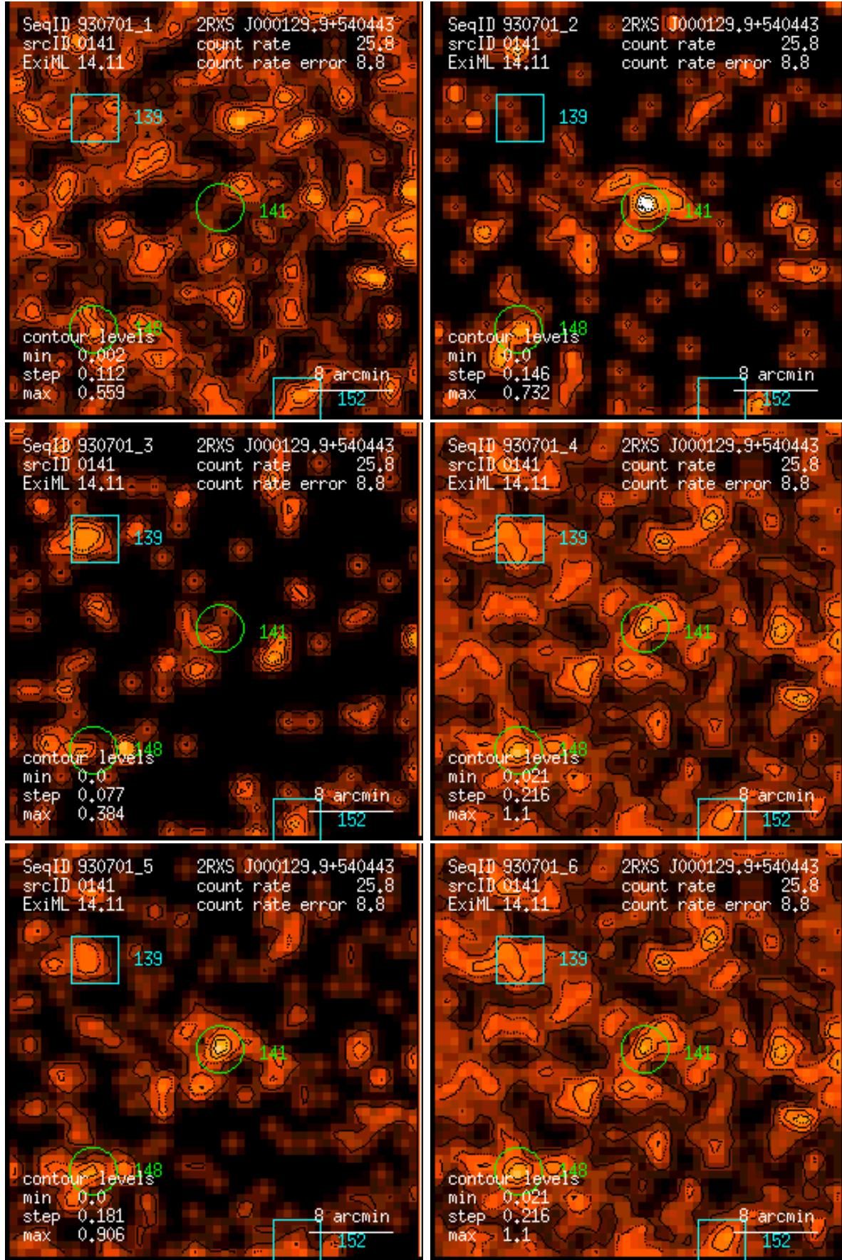
Figure 141: RASS 930701: detection 0141: band rate images, Gaussian filter: (1) PSPC channels 11 – 41, (2) 52 – 90, (3) 91 – 201, (4) 11 – 235, (5) 52 – 201, (6) 11 – 201. Broad band rates in counts/ks. Band rate contour levels in counts/ks/arcmin 2 .
