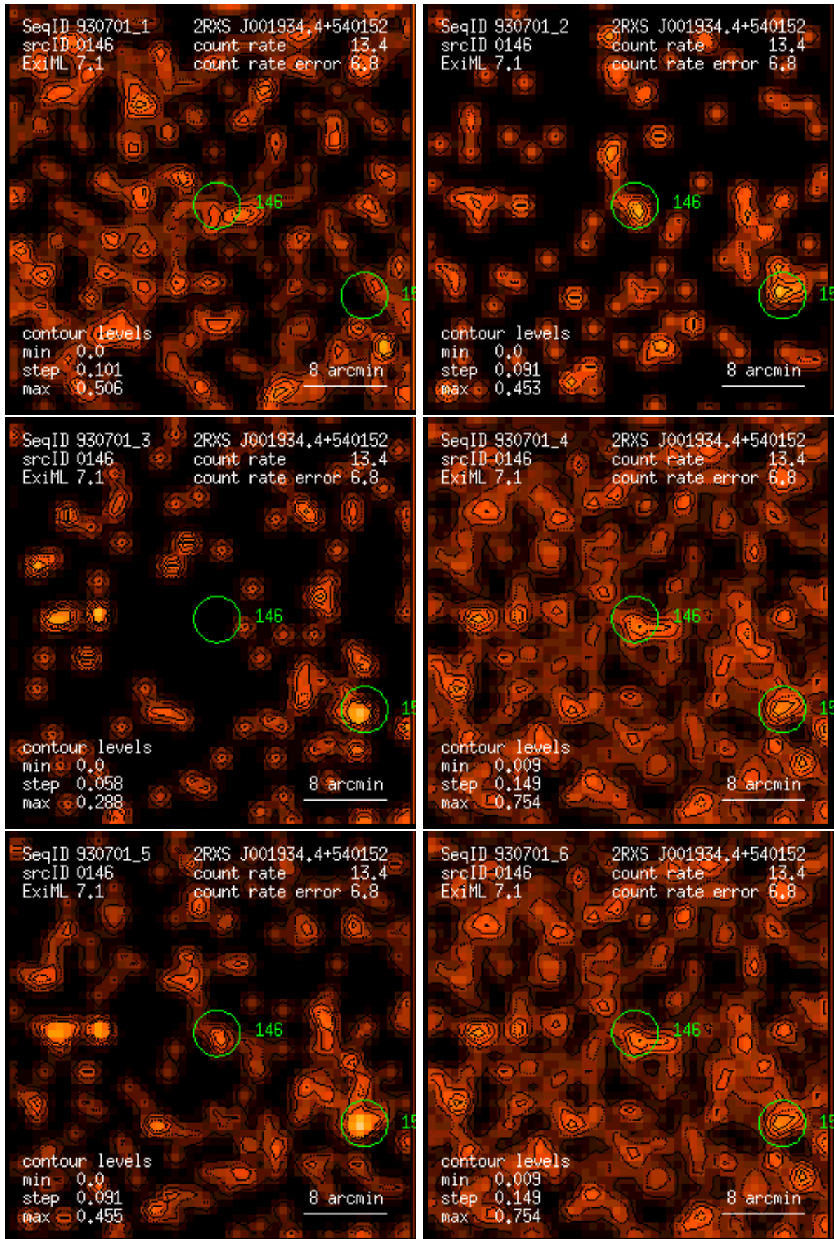
Figure 146: RASS 930701: detection 0146: band rate images, Gaussian filter: (1) PSPC channels 11 – 41, (2) 52 – 90, (3) 91 – 201, (4) 11 – 235, (5) 52 – 201, (6) 11 – 201. Broad band rates in counts/ks. Band rate contour levels in counts/ks/arcmin 2 .
