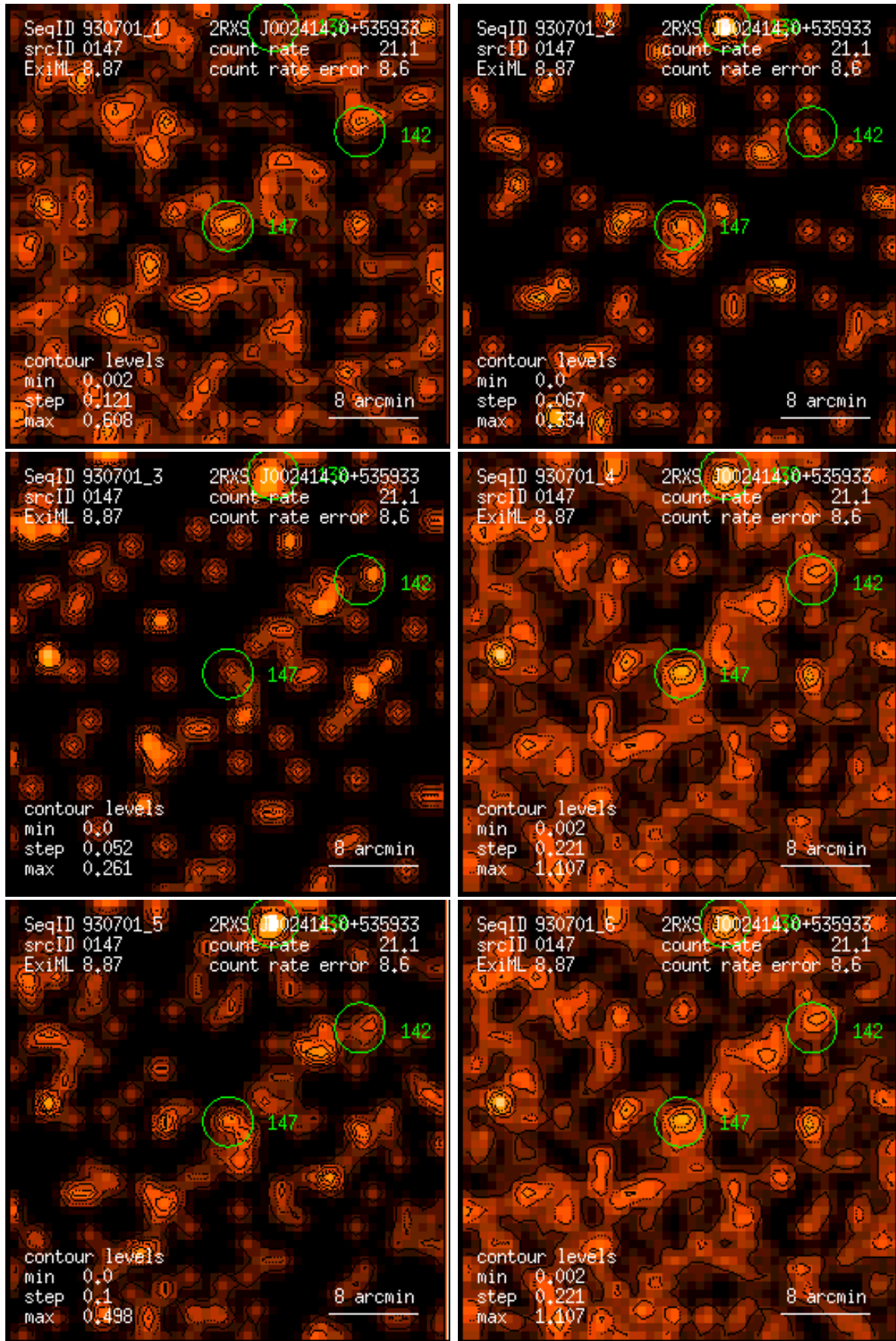
Figure 147: RASS 930701: detection 0147: band rate images, Gaussian filter: (1) PSPC channels 11 – 41, (2) 52 – 90, (3) 91 – 201, (4) 11 – 235, (5) 52 – 201, (6) 11 – 201. Broad band rates in counts/ks. Band rate contour levels in counts/ks/arcmin 2 .
