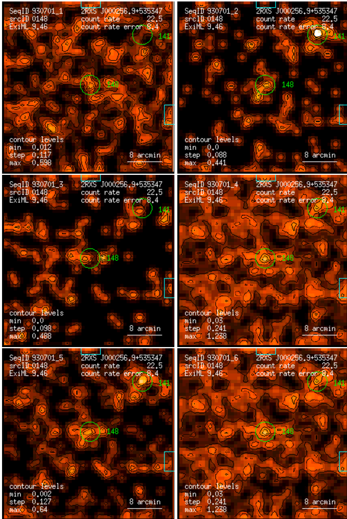
Figure 148: RASS 930701: detection 0148: band rate images, Gaussian filter: (1) PSPC channels 11 – 41, (2) 52 – 90, (3) 91 – 201, (4) 11 – 235, (5) 52 – 201, (6) 11 – 201. Broad band rates in counts/ks. Band rate contour levels in counts/ks/arcmin 2 .
