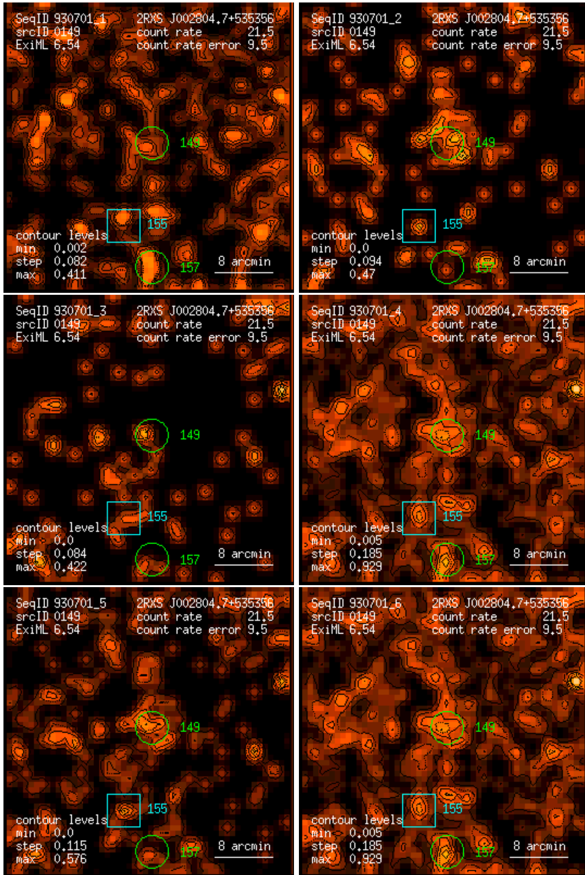
Figure 149: RASS 930701: detection 0149: band rate images, Gaussian filter: (1) PSPC channels 11 – 41, (2) 52 – 90, (3) 91 – 201, (4) 11 – 235, (5) 52 – 201, (6) 11 – 201. Broad band rates in counts/ks. Band rate contour levels in counts/ks/arcmin 2 .
