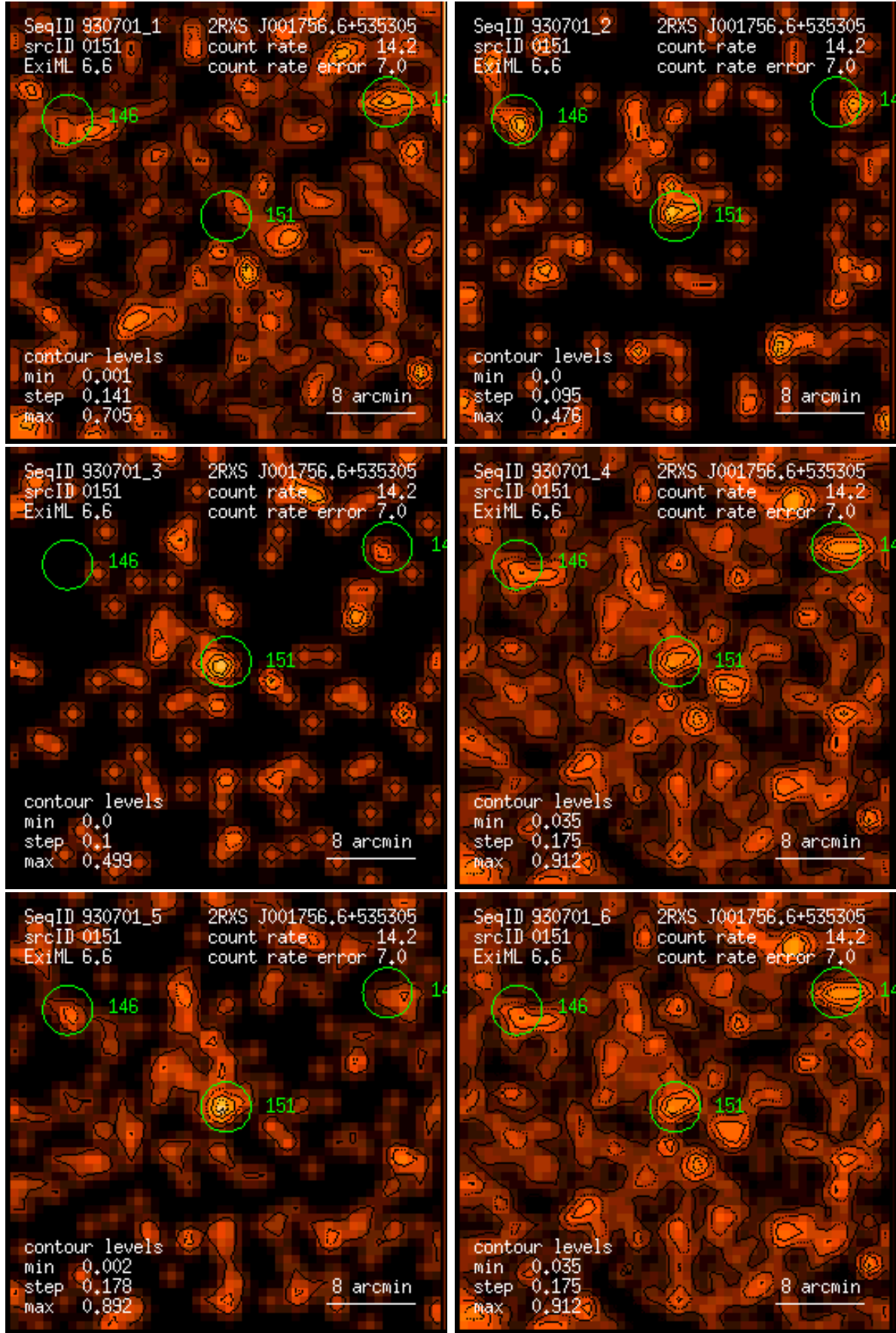
Figure 151: RASS 930701: detection 0151: band rate images, Gaussian filter: (1) PSPC channels 11 – 41, (2) 52 – 90, (3) 91 – 201, (4) 11 – 235, (5) 52 – 201, (6) 11 – 201. Broad band rates in counts/ks. Band rate contour levels in counts/ks/arcmin 2 .
