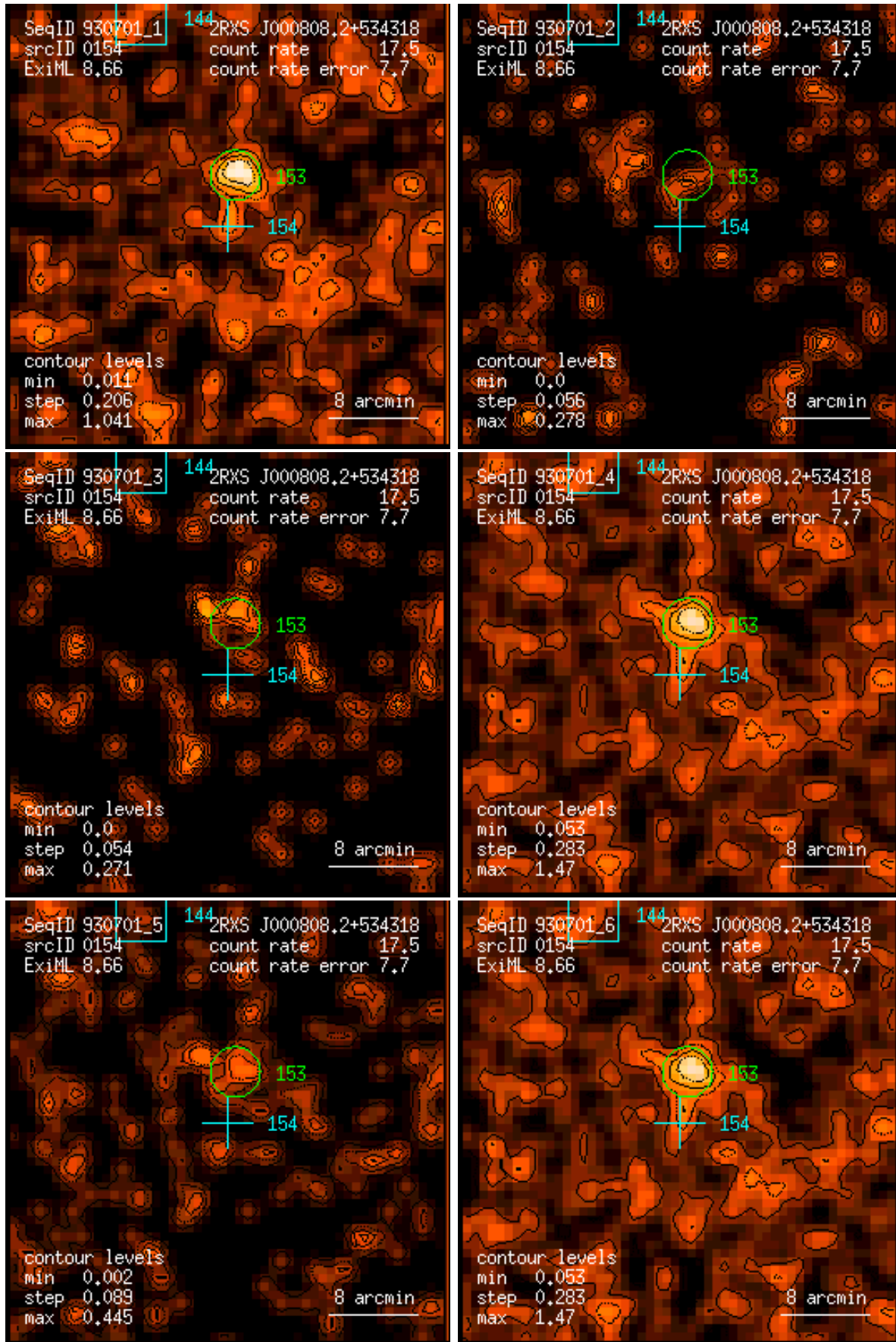
Figure 154: RASS 930701: detection 0154: band rate images, Gaussian filter: (1) PSPC channels 11 – 41, (2) 52 – 90, (3) 91 – 201, (4) 11 – 235, (5) 52 – 201, (6) 11 – 201. Broad band rates in counts/ks. Band rate contour levels in counts/ks/arcmin 2 .
