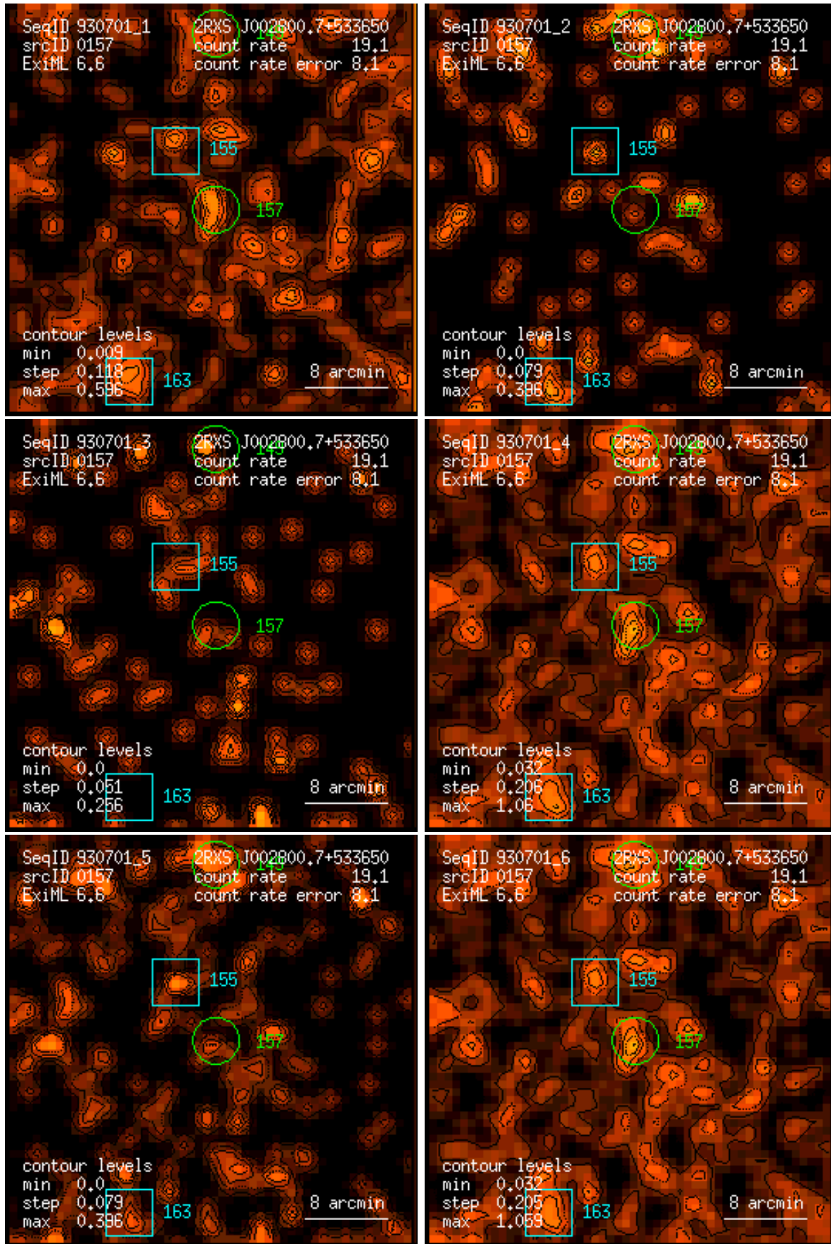
Figure 157: RASS 930701: detection 0157: band rate images, Gaussian filter: (1) PSPC channels 11 – 41, (2) 52 – 90, (3) 91 – 201, (4) 11 – 235, (5) 52 – 201, (6) 11 – 201. Broad band rates in counts/ks. Band rate contour levels in counts/ks/arcmin 2 .
