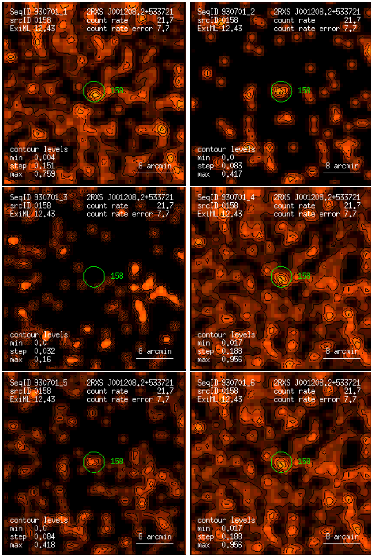
Figure 158: RASS 930701: detection 0158: band rate images, Gaussian filter: (1) PSPC channels 11 – 41, (2) 52 – 90, (3) 91 – 201, (4) 11 – 235, (5) 52 – 201, (6) 11 – 201. Broad band rates in counts/ks. Band rate contour levels in counts/ks/arcmin 2 .
