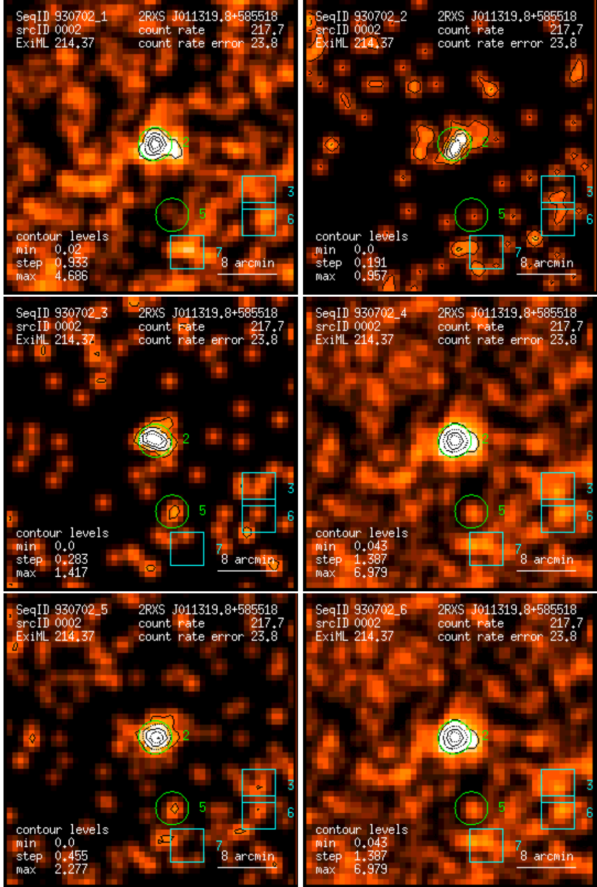
Figure 2: RASS 930702: detection 0002: band rate images, Gaussian filter: (1) PSPC channels 11 – 41, (2) 52 – 90, (3) 91 – 201, (4) 11 – 235, (5) 52 – 201, (6) 11 – 201. Broad band rates in counts/ks. Band rate contour levels in counts/ks/arcmin 2 .
