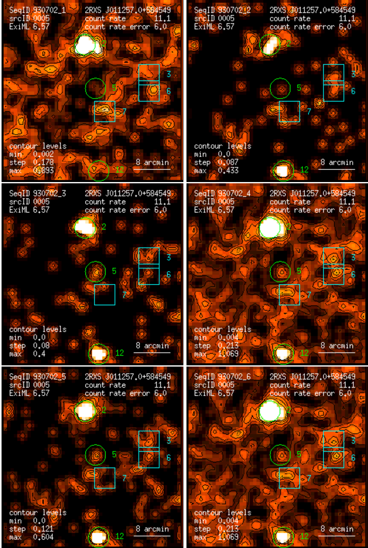
Figure 5: RASS 930702: detection 0005: band rate images, Gaussian filter: (1) PSPC channels 11 – 41, (2) 52 – 90, (3) 91 – 201, (4) 11 – 235, (5) 52 – 201, (6) 11 – 201. Broad band rates in counts/ks. Band rate contour levels in counts/ks/arcmin 2 .
