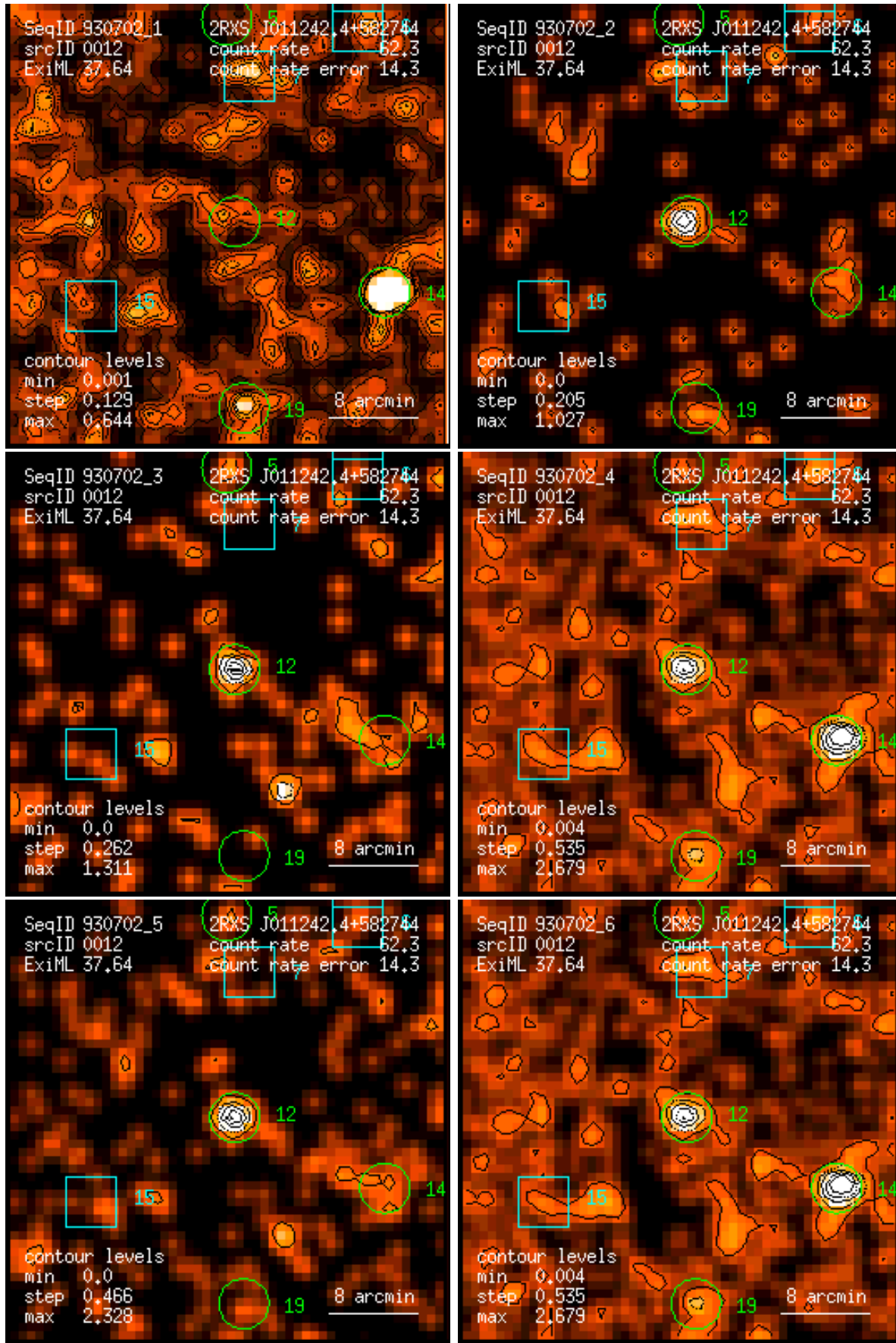
Figure 12: RASS 930702: detection 0012: band rate images, Gaussian filter: (1) PSPC channels 11 – 41, (2) 52 – 90, (3) 91 – 201, (4) 11 – 235, (5) 52 – 201, (6) 11 – 201. Broad band rates in counts/ks. Band rate contour levels in counts/ks/arcmin 2 .
