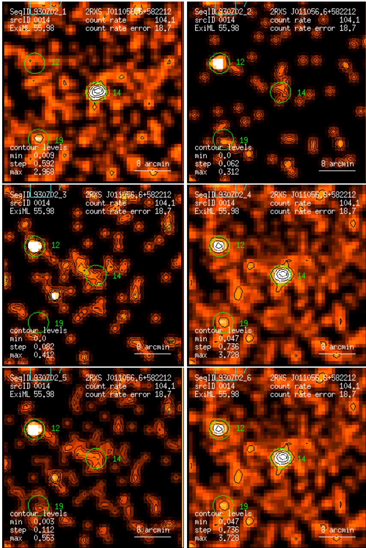
Figure 14: RASS 930702: detection 0014: band rate images, Gaussian filter: (1) PSPC channels 11 – 41, (2) 52 – 90, (3) 91 – 201, (4) 11 – 235, (5) 52 – 201, (6) 11 – 201. Broad band rates in counts/ks. Band rate contour levels in counts/ks/arcmin 2 .
