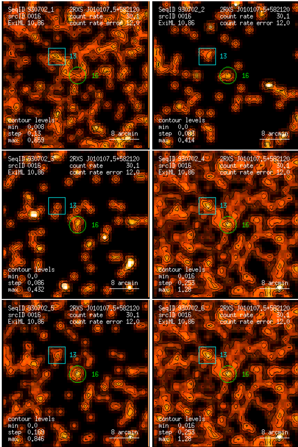
Figure 16: RASS 930702: detection 0016: band rate images, Gaussian filter: (1) PSPC channels 11 – 41, (2) 52 – 90, (3) 91 – 201, (4) 11 – 235, (5) 52 – 201, (6) 11 – 201. Broad band rates in counts/ks. Band rate contour levels in counts/ks/arcmin 2 .
