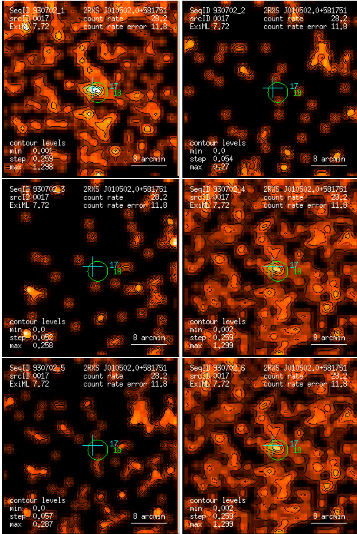
Figure 17: RASS 930702: detection 0017: band rate images, Gaussian filter: (1) PSPC channels 11 – 41, (2) 52 – 90, (3) 91 – 201, (4) 11 – 235, (5) 52 – 201, (6) 11 – 201. Broad band rates in counts/ks. Band rate contour levels in counts/ks/arcmin 2 .
