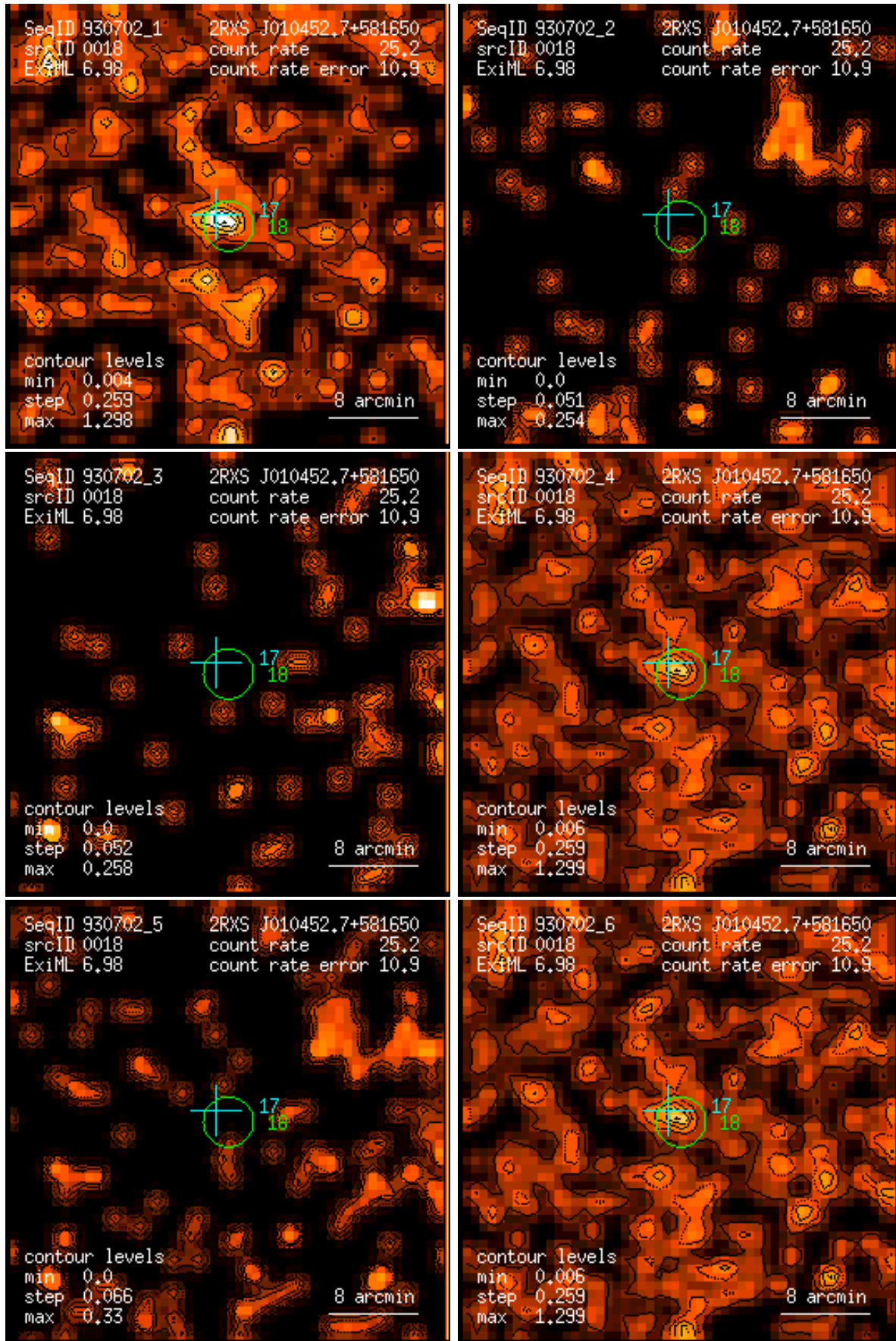
Figure 18: RASS 930702: detection 0018: band rate images, Gaussian filter: (1) PSPC channels 11 – 41, (2) 52 – 90, (3) 91 – 201, (4) 11 – 235, (5) 52 – 201, (6) 11 – 201. Broad band rates in counts/ks. Band rate contour levels in counts/ks/arcmin 2 .
